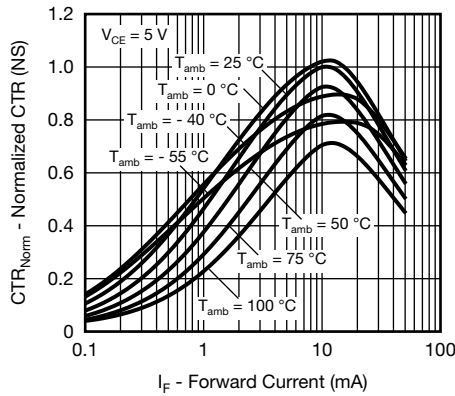
Fig. 9 - Normalized CTR (NS) vs. Forward Current
